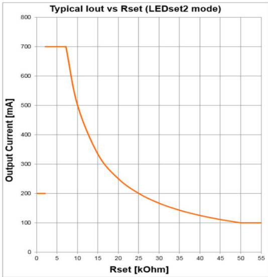
OT FIT 100220-240700 D NFC IND Typical Iout vs Rset (LEDset2 mode)
