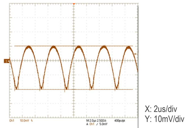
( V_{IN} = 24V , I_{OUT} = 3.5A , C_{OUT} = 110\mu F , ScopeBW = 20MHz) Figure 14. Output Ripple and Noise
