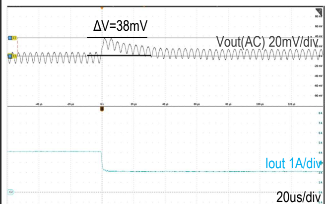
( V_{IN} = 12.0\text{V} , C_{OUT} = 110\mu\text{F} , I_{OUT} = 4.0\text{A} to 2.0\text{A} , 1\text{A}/\mu\text{s} ) Figure 10. Step Load Transient Response
