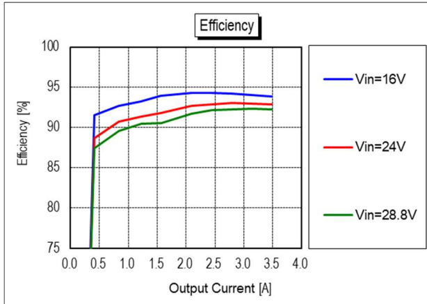
Figure 23. Efficiency vs. Load Current and Line Voltage
