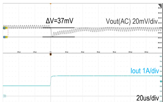
( V_{IN} = 12.0V , C_{OUT} = 110\mu F , I_{OUT} = 2.0A to 4.0A , 1A/us ) Figure 21. Step Load Transient Response
