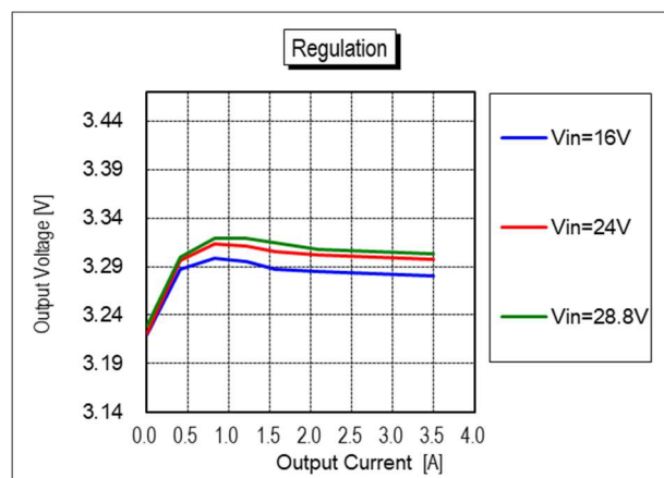
Figure 12. V_{OUT} vs. Load Current and Line Voltage
