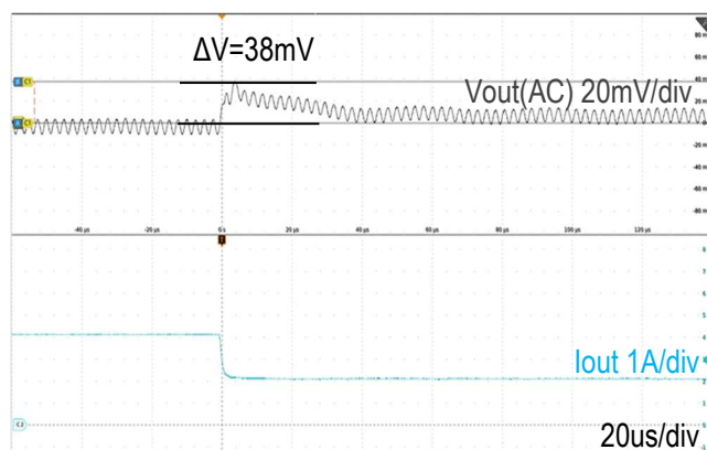
( V_{IN} = 12.0V , C_{OUT} = 110\mu F , I_{OUT} = 4.0A to 2.0A , 1A/us ) Figure 22. Step Load Transient Response
