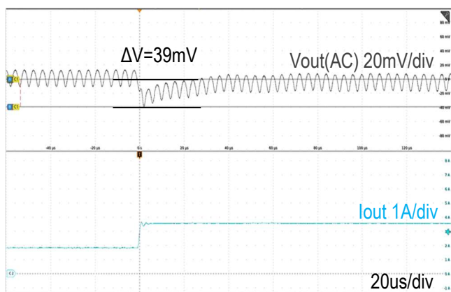
( V_{IN} = 24.0V , C_{OUT} = 110\mu F , I_{OUT} = 1.75A to 3.5A , 1A/\mu s ) Figure 15. Step Load Transient Response
