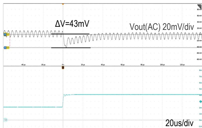
( V_{IN} = 12.0\text{V} , C_{OUT} = 110\mu\text{F} , I_{OUT} = 2.0\text{A} to 4.0\text{A} , 1\text{A}/\mu\text{s} ) Figure 9. Step Load Transient Response
