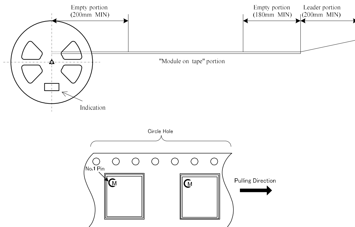
Figure 41. Tape Specifications
