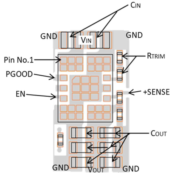
Figure 35. Example of Pattern Layout (Top View)
