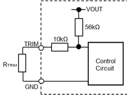
Figure 33. TRIM Internal Circuit Diagram
