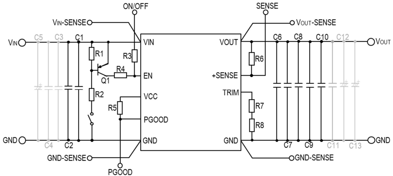
Figure 34. Application Circuit
