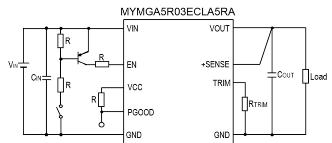
Figure 2. Simplified Circuit Diagram
