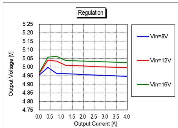
Figure 18. V_{OUT} vs. Load Current and Line Voltage
