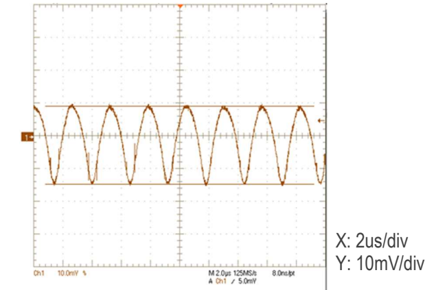
( V_{IN} = 24V , I_{OUT} = 3.5A , C_{OUT} = 100\mu F , ScopeBW = 20MHz) Figure 26. Output Ripple and Noise
