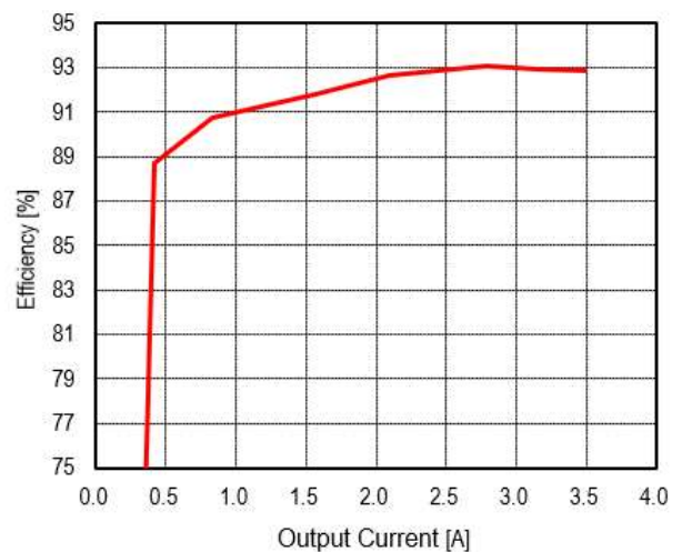
Figure 1. Efficiency Curve
