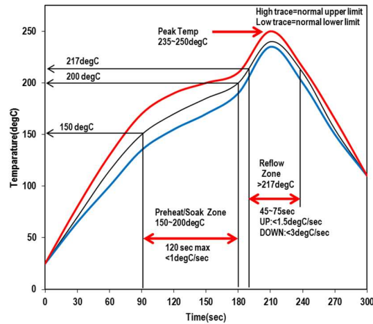
Figure 42. Recommended Lead-free Solder Reflow Profile
