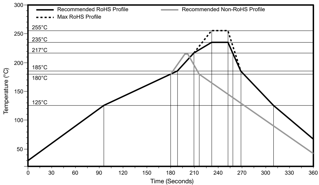
Figure 11. Solder Profile for the ANT-868-VHETH Antenna
