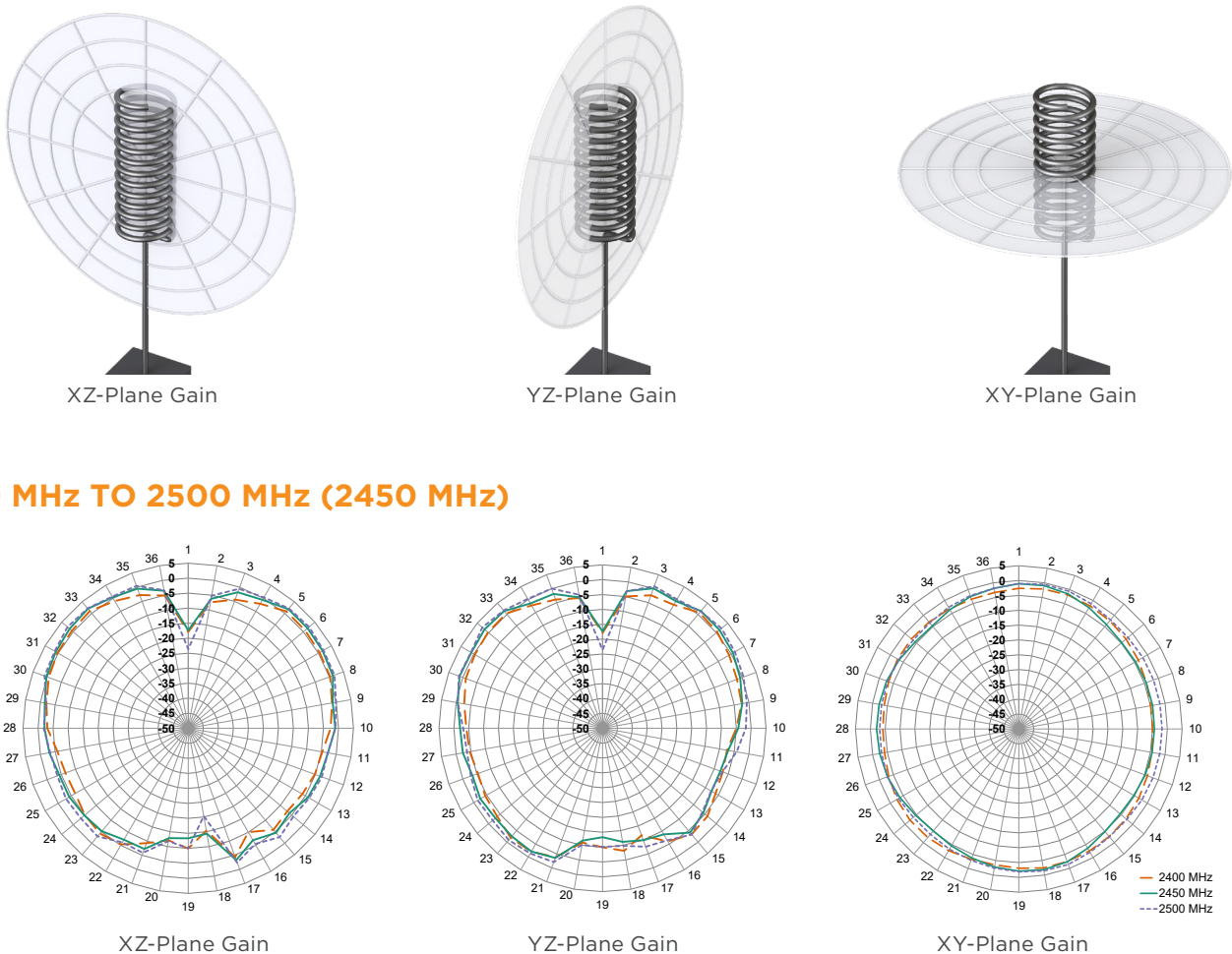
Figure 7. Radiation Patterns for ANT-2.4-VHETH
