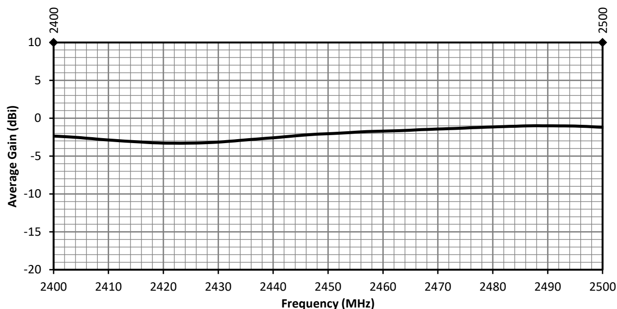
Figure 5. ANT-2.4-VHETH Antenna Average Gain
