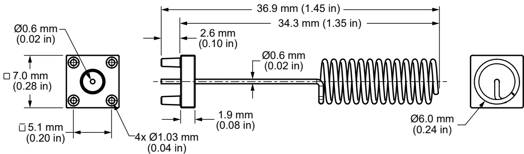
Figure 1. ANT-2.4-VHETH Antenna Dimensions
