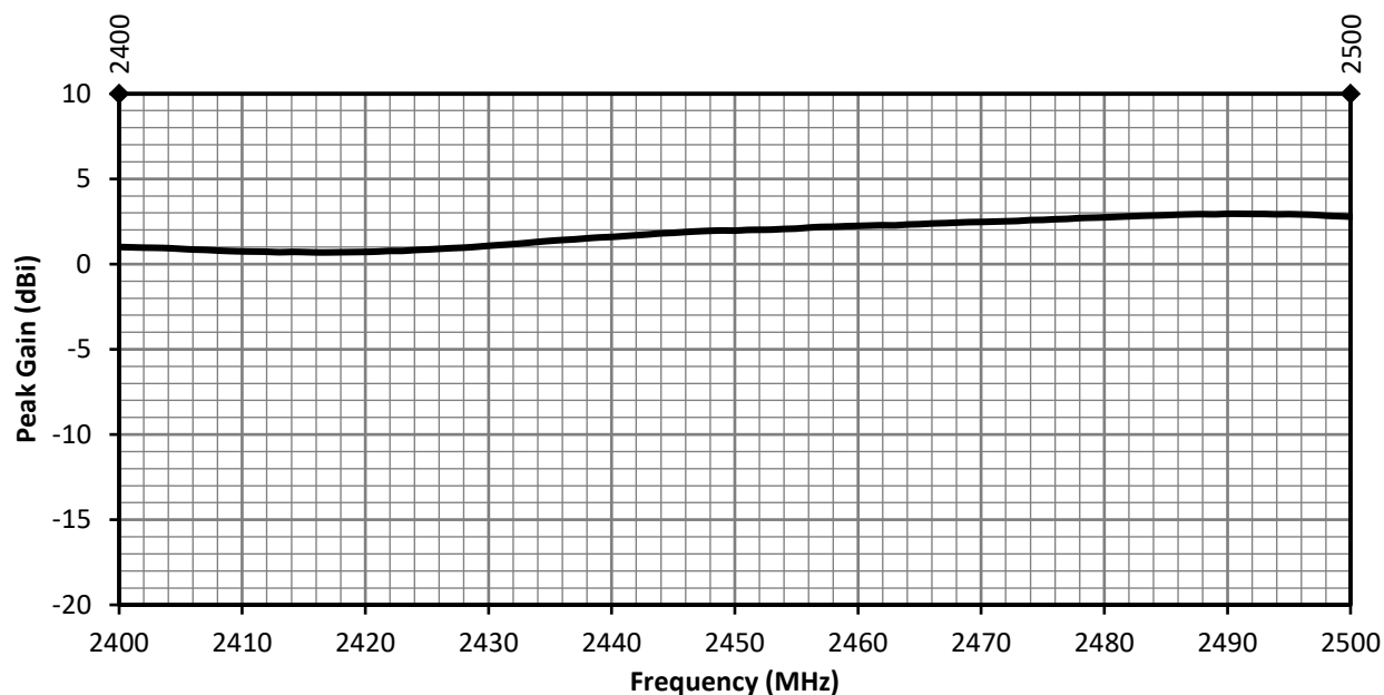
Figure 4. ANT-2.4-VHETH Antenna Peak Gain
