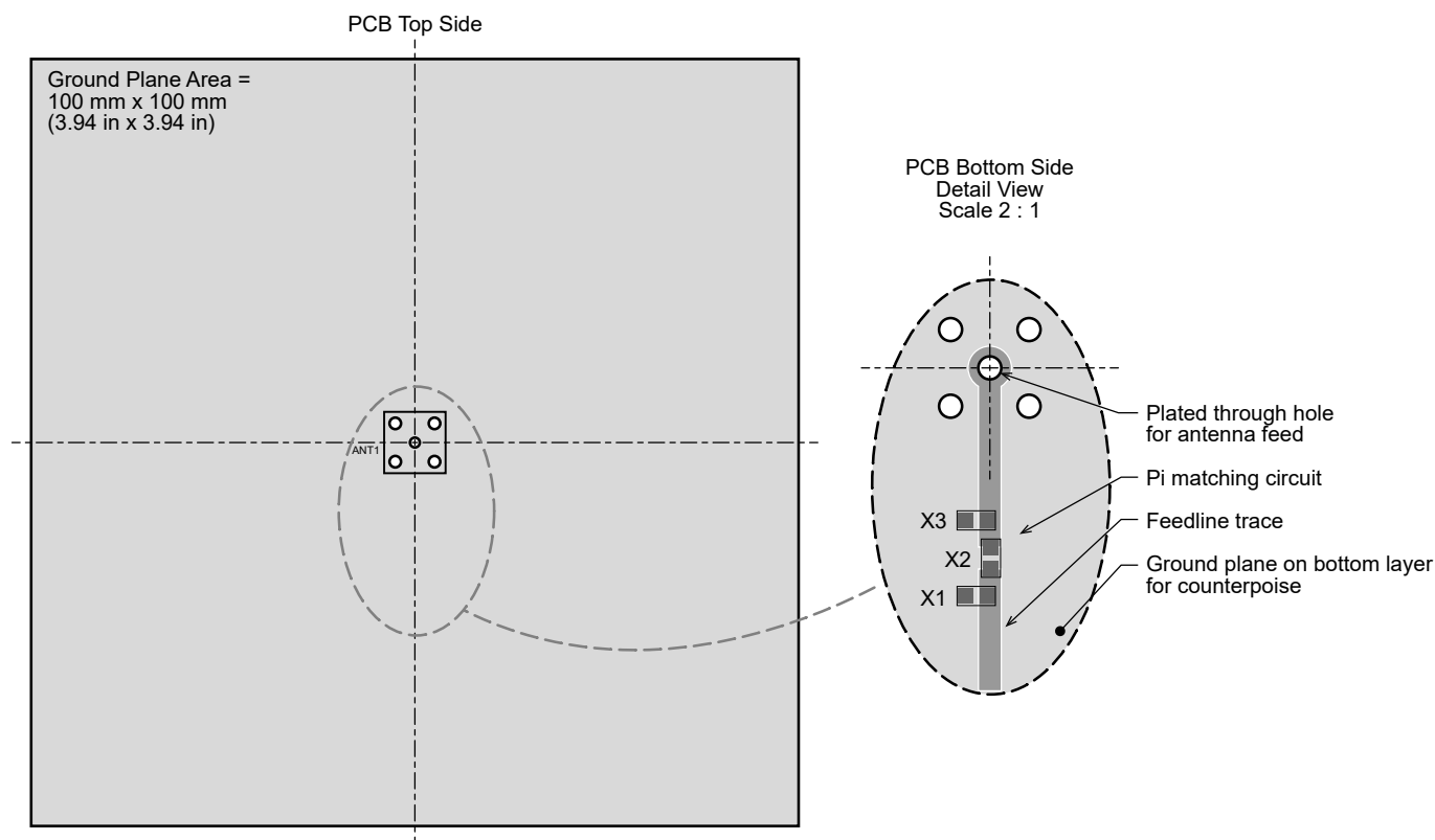
Figure 8. ANT-2.4-VHETH Recommended Layout
