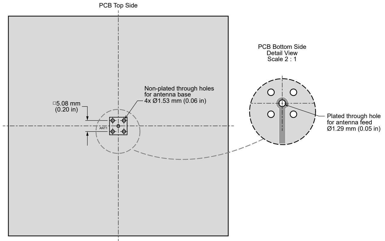
Figure 10. ANT-2.4-VHETH Antenna Placement on PCB
