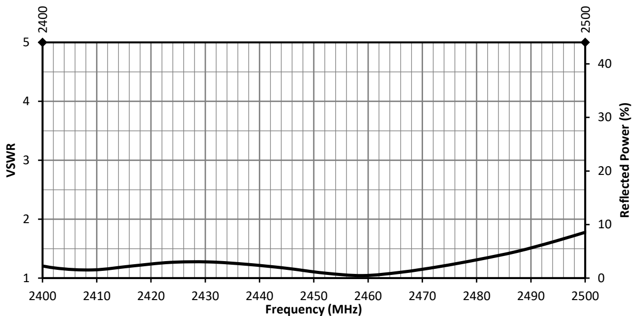
Figure 2. ANT-2.4-VHETH Antenna VSWR
