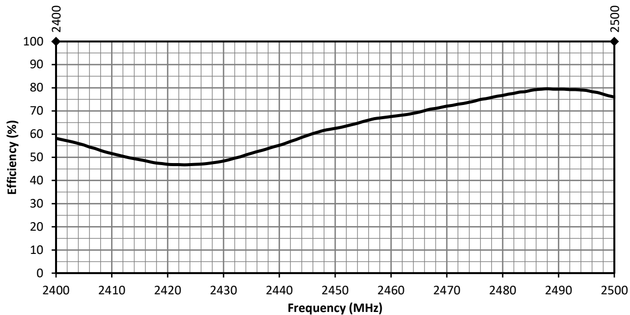
Figure 6. ANT-2.4-VHETH Antenna Radiation Efficiency
