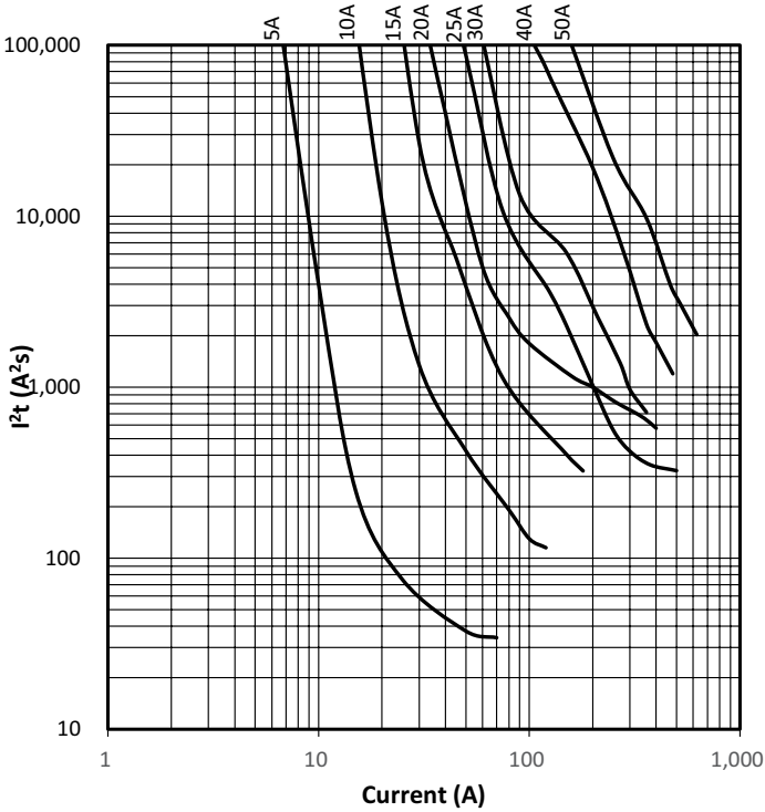
I 2 t vs. current curve
