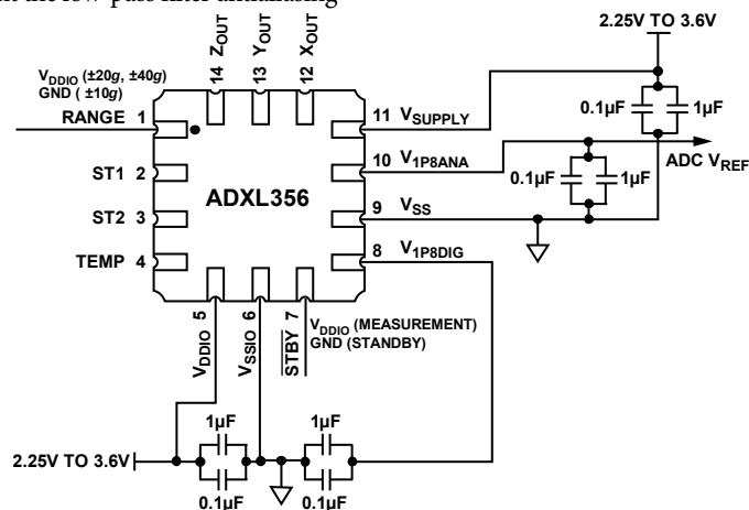
Figure 58. ADXL356 Application Circuit
