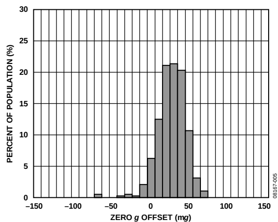
Figure 5. Y-Axis Zero g Offset at 25°C, V_S = 2.6\text{ V}
