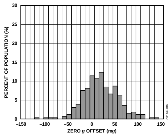
Figure 9. Z-Axis Zero g Offset at 25°C, V_S = 1.8\text{ V}
