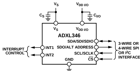
Figure 44. Applications Diagram
