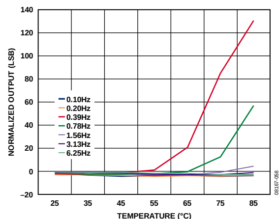
Figure 59. Typical Z-Axis Output vs. Temperature at Lower Data Rates, Normalized to 100 Hz Output Data Rate, V_S = 2.6 V
