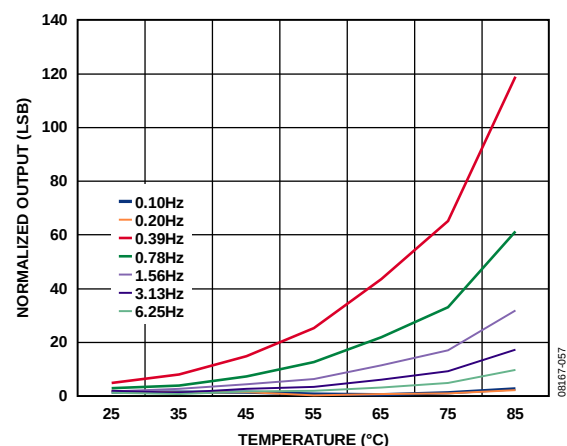
Figure 58. Typical Y-Axis Output vs. Temperature at Lower Data Rates, Normalized to 100 Hz Output Data Rate, V_S = 2.6 V
