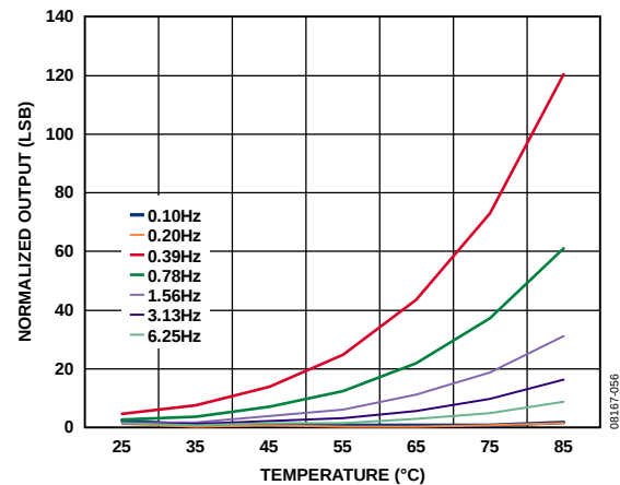
Figure 57. Typical X-Axis Output vs. Temperature at Lower Data Rates, Normalized to 100 Hz Output Data Rate, V_S = 2.6 V
