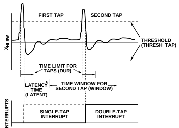
Figure 46. Tap Interrupt Function with Valid Single and Double Taps
