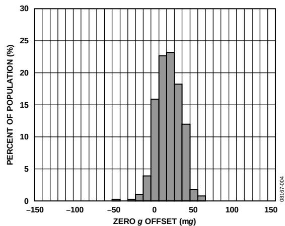
Figure 4. X-Axis Zero g Offset at 25°C, V_S = 2.6\text{ V}
