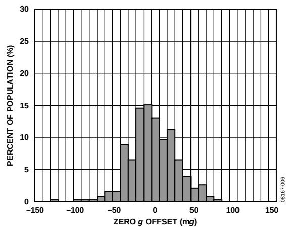
Figure 6. Z-Axis Zero g Offset at 25°C, V_S = 2.6\text{ V}
