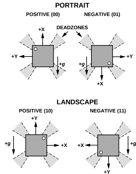
Figure 50. 2D Orientation with Corresponding Codes
