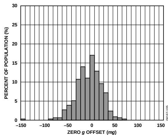
Figure 8. Y-Axis Zero g Offset at 25°C, V_S = 1.8\text{ V}
