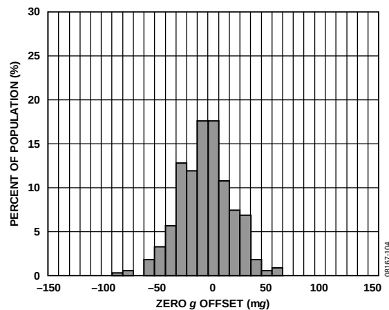
Figure 7. X-Axis Zero g Offset at 25°C, V_S = 1.8\text{ V}
