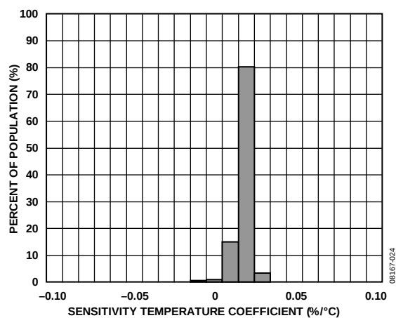
Figure 24. Z-Axis Sensitivity Temperature Coefficient, V_S = 2.6\text{ V}
