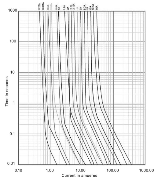
Average time current (I-T curves)
