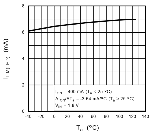
Fig. 12.11 I_{LIM(LED)} - T_a
