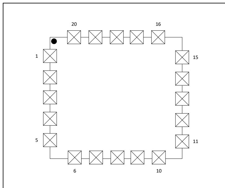
Figure 3: Pin Diagram of AS7265x (Top View)
