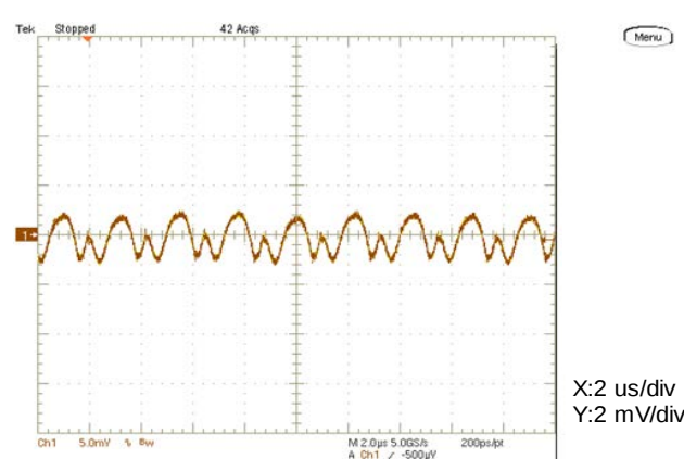
( V_{IN} = 12\text{V} , I_{OUT} = 16\text{A} , C_{OUT} = 660\mu\text{F} , ScopeBW = 20MHz) Figure 8. Output Ripple and Noise
