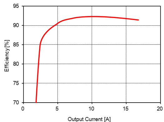
Figure 1. Efficiency Curve
