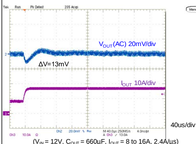
( V_{IN} = 12\text{V} , C_{OUT} = 660\mu\text{F} , I_{OUT} = 8 to 16\text{A} , 2.4\mu\text{s} ) Figure 9. Step Load Transient Response
