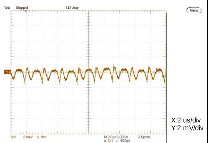
( V_{IN} = 12V , I_{OUT} = 16A , C_{OUT} = 660\mu F , ScopeBW = 20MHz) Figure 20. Output Ripple and Noise
