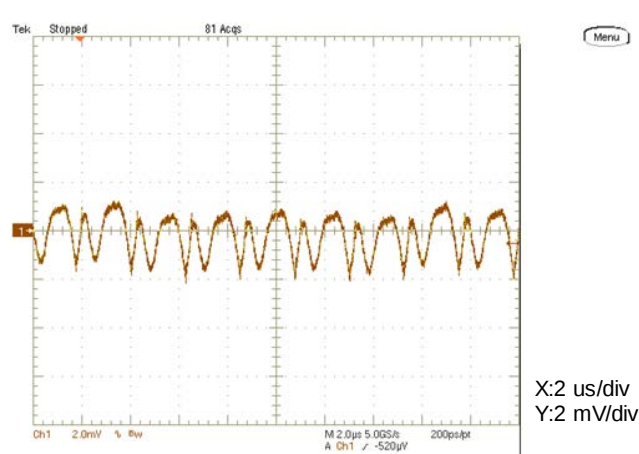
( V_{IN} = 12V , I_{OUT} = 16A , C_{OUT} = 660\mu F , ScopeBW = 20MHz) Figure14. Output Ripple and Noise
