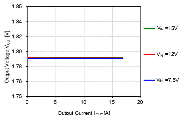
Figure 6. V_{OUT} vs. Load Current and Line Voltage
