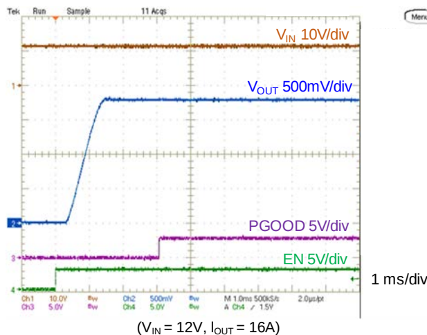
( V_{IN} = 12V , I_{OUT} = 16A ) Figure 19. On/Off Enable wave form
