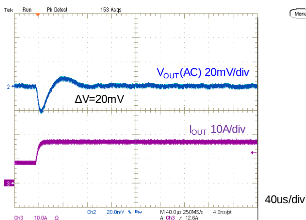
( V_{IN} = 12V , C_{OUT} = 660\mu F , I_{OUT} = 8 to 16A , 2.4A/\mu s ) Figure 21. Step Load Transient Response
