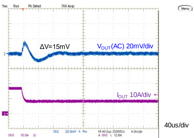
( V_{IN} = 12V , C_{OUT} = 660\mu F , I_{OUT} = 16 to 8A , 2.4A/\mu s ) Figure 16. Step Load Transient Response
