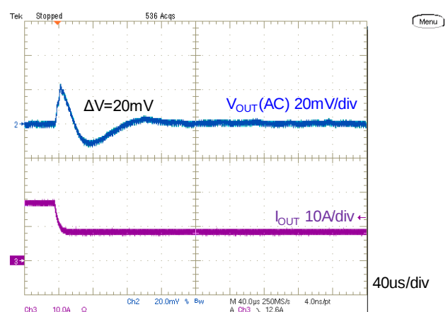
( V_{IN} = 12V , C_{OUT} = 660\mu F , I_{OUT} = 16 to 8A , 2.4A/\mu s ) Figure 22. Step Load Transient Response
