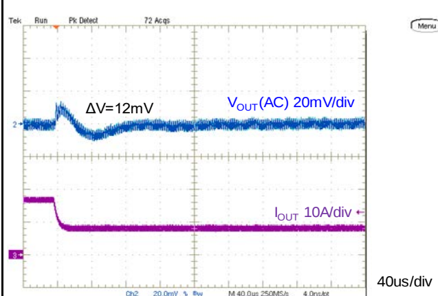
( V_{IN} = 12\text{V} , C_{OUT} = 660\mu\text{F} , I_{OUT} = 16 to 8\text{A} , 2.4\mu\text{s} ) Figure 10. Step Load Transient Response
