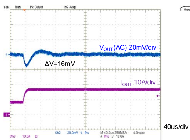
( V_{IN} = 12V , C_{OUT} = 660\mu F , I_{OUT} = 8 to 16A , 2.4A/\mu s ) Figure 15. Step Load Transient Response
