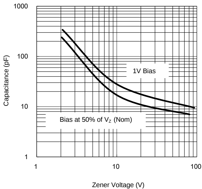
Fig.3 Typical Capacitance
