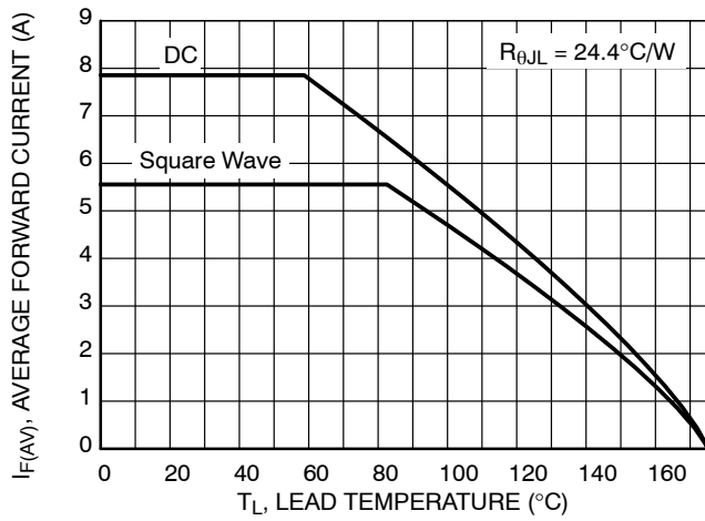
Figure 7. Current Derating per Diode for NRVTSF5100E
