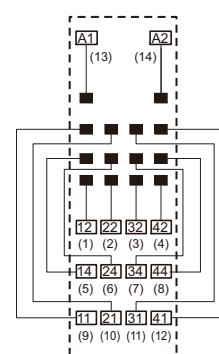
Terminal Arrangement/Internal Connection Diagram
