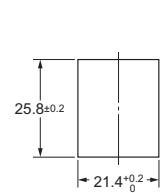
Mounting Hole Dimensions
