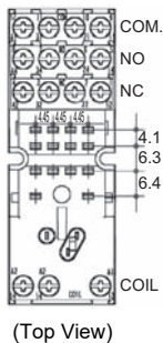
Terminal arrangement/ Internal connections/ mounting holes
