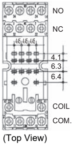
Terminal arrangement/ Internal connections/ mounting holes
