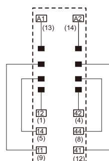
Terminal Arrangement/Internal Connection Diagram
