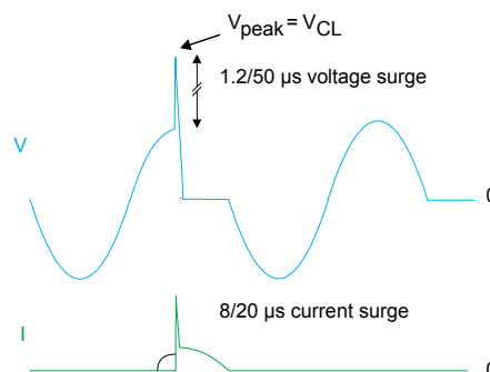
Figure 15. Typical voltage and current waveforms across the ACST1220H-8H during IEC61000-4-5 standard test
