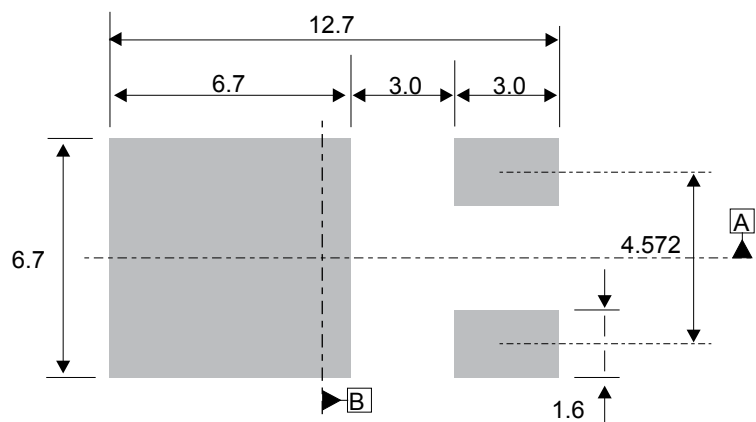
Figure 18. DPAK recommended footprint (dimensions are in mm)
