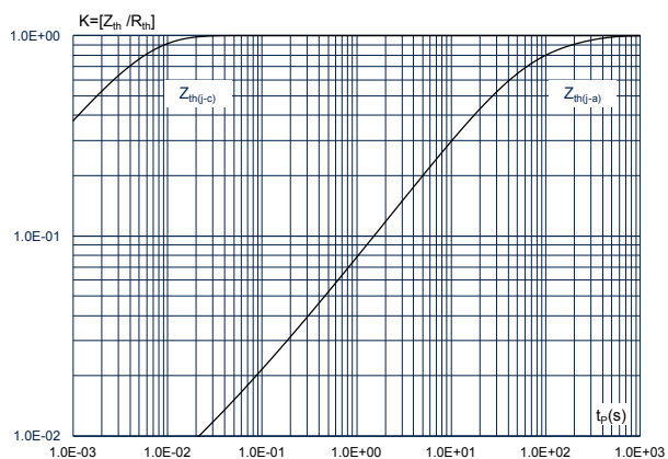
Figure 13. Relative variation of thermal impedance versus pulse duration
