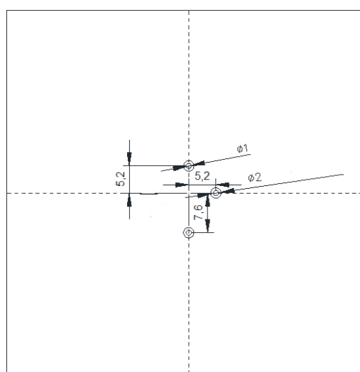
BOTTOM SIDE OF PCB
