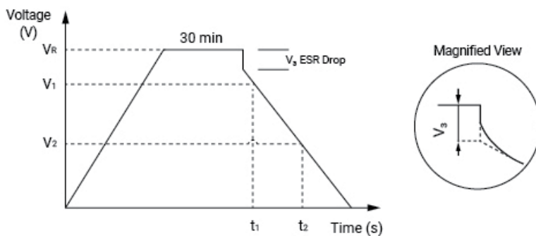
Figure 1; Constant current discharge method for capacitance, and V3 voltage drop for DCESR.
