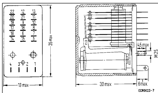
Size III case - 6 Changeover & 4 Changeover heavy duty V23054-E
