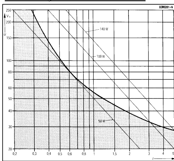
DC switching limit curve for F1 contacts
