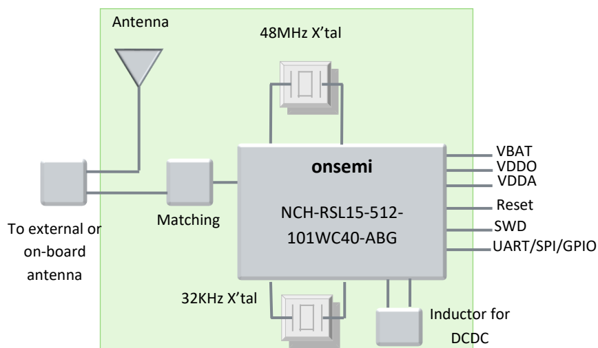
Figure 1: Type 2EG Block Diagram
