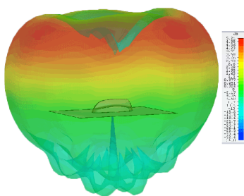
3D Gain Plot Side (1800MHz)
