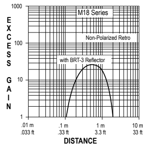
Excess Gain
