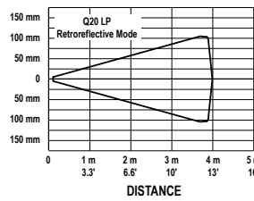
Beam Pattern
