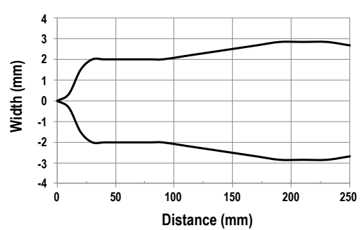
Beam Pattern
