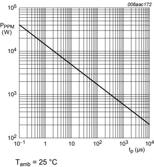
Fig. 3. Rated peak pulse power as a function of pulse duration; typical values
