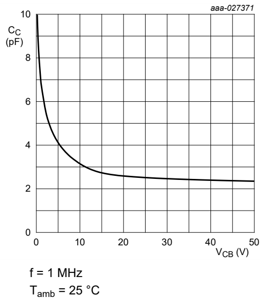
Fig. 16. BC817K-16H-Q: Collector capacitance as a function of collector-base voltage; typical values
