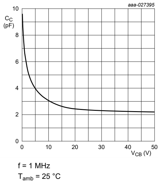
Fig. 40. BC817K-40H-Q: Collector capacitance as a function of collector-base voltage; typical values
