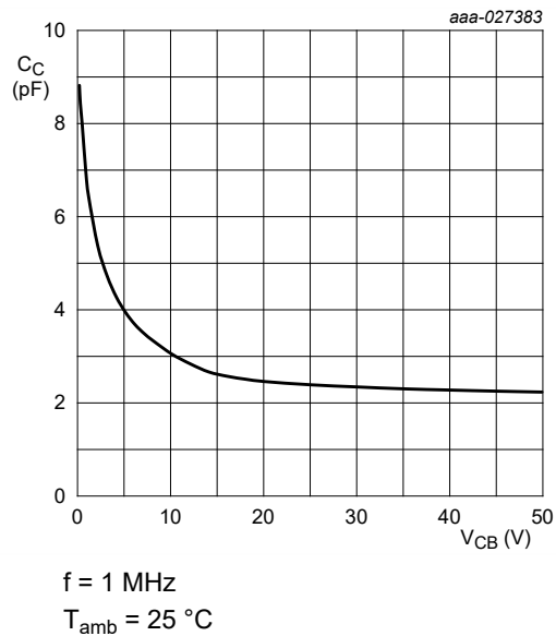
Fig. 28. BC817K-25H-Q: Collector capacitance as a function of collector-base voltage; typical values
