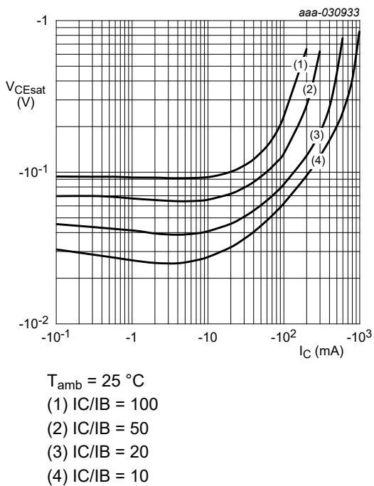
Fig. 23. BC806-25H-Q: Collector-emitter saturation voltage as a function of collector current; typical values
