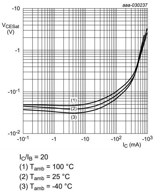
Fig. 22. BC806-25H-Q: Collector-emitter saturation voltage as a function of collector current; typical values
