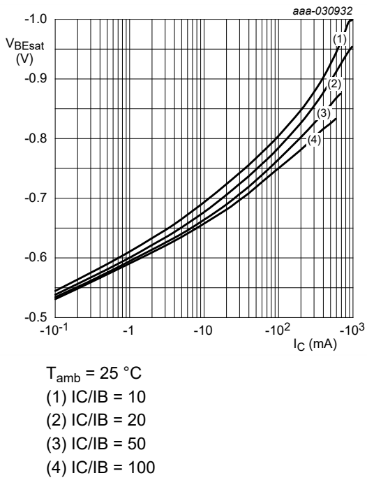
Fig. 21. BC806-25H-Q: Base-emitter saturation voltage as a function of collector current; typical values
