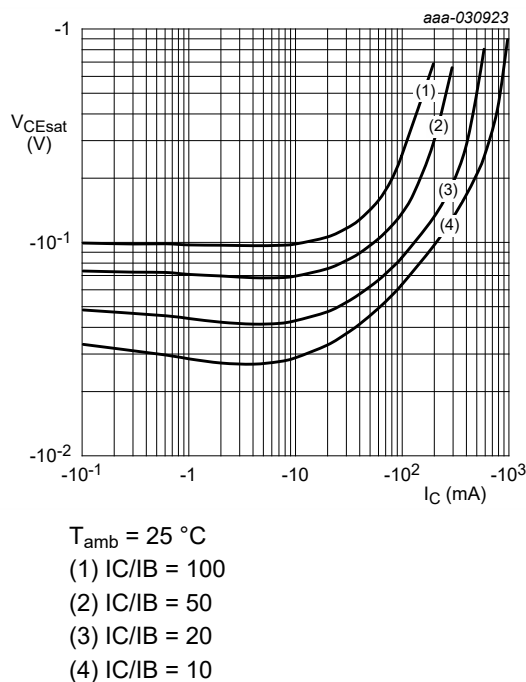
Fig. 11. BC806-16H-Q: Collector-emitter saturation voltage as a function of collector current; typical values
