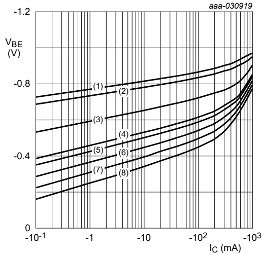
V_{CE} = -5\text{ V} (1) T_{amb} = -55\text{ °C} (2) T_{amb} = -40\text{ °C} (3) T_{amb} = 25\text{ °C} (4) T_{amb} = 85\text{ °C} (5) T_{amb} = 100\text{ °C} (6) T_{amb} = 125\text{ °C} (7) T_{amb} = 150\text{ °C} (8) T_{amb} = 175\text{ °C}
