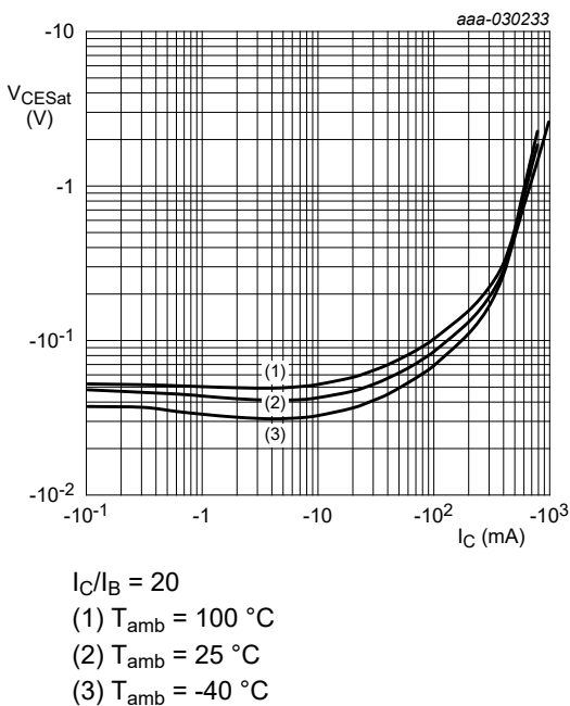
Fig. 10. BC806-16H-Q: Collector-emitter saturation voltage as a function of collector current; typical values
