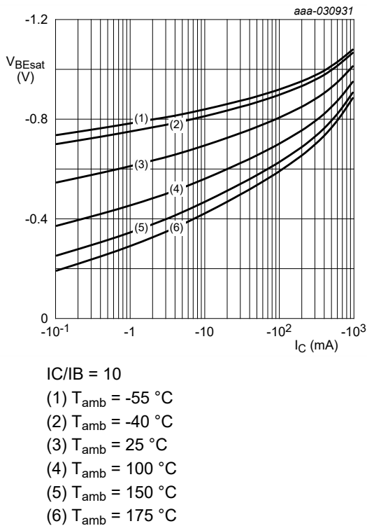
Fig. 20. BC806-25H-Q: Base-emitter saturation voltage as a function of collector current; typical values
