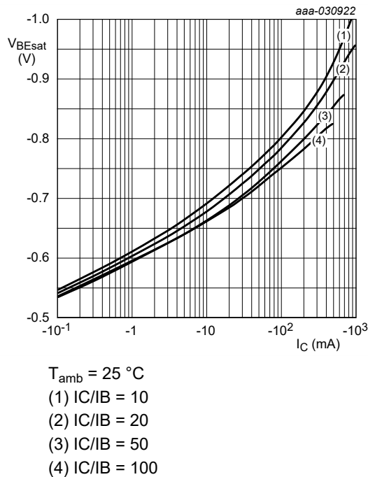
Fig. 9. BC806-16H-Q: Base-emitter saturation voltage as a function of collector current; typical values
