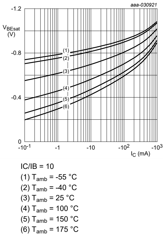
Fig. 8. BC806-16H-Q: Base-emitter saturation voltage as a function of collector current; typical values
