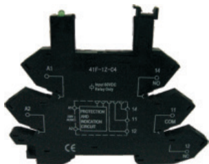
Green LED Diode indicates operate status of relay
