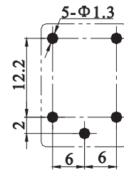
PCB Mounting Dimensions mm
