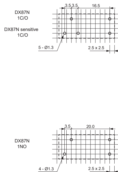
PCB Mounting Holes Dimensions mm (bottom view)
