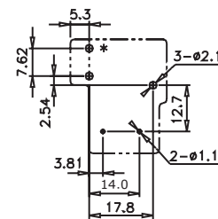
PCB Mounting Dimensions mm
