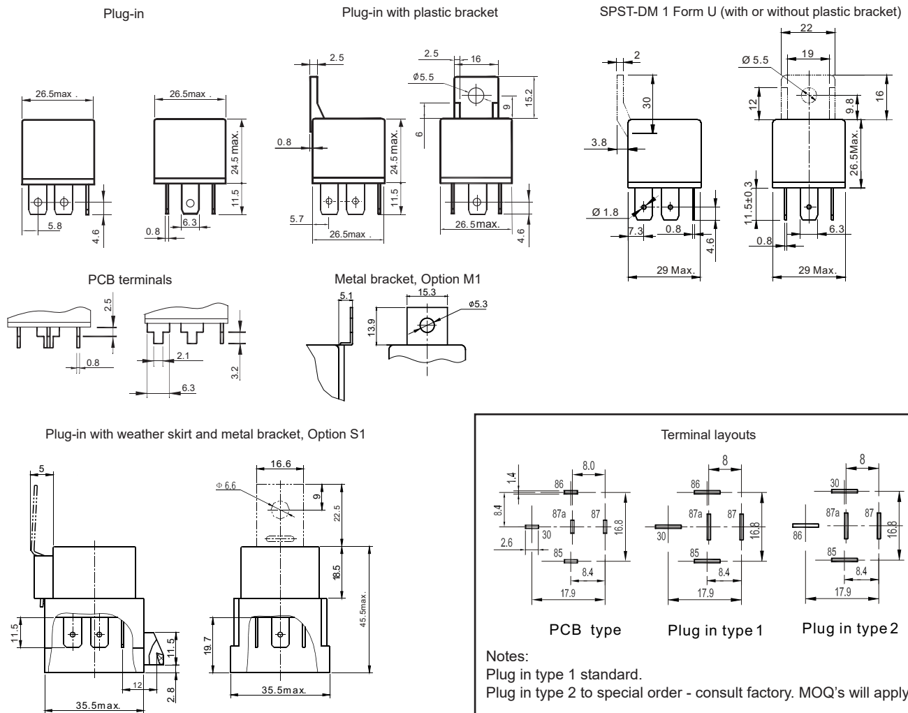
Dimensions mm
