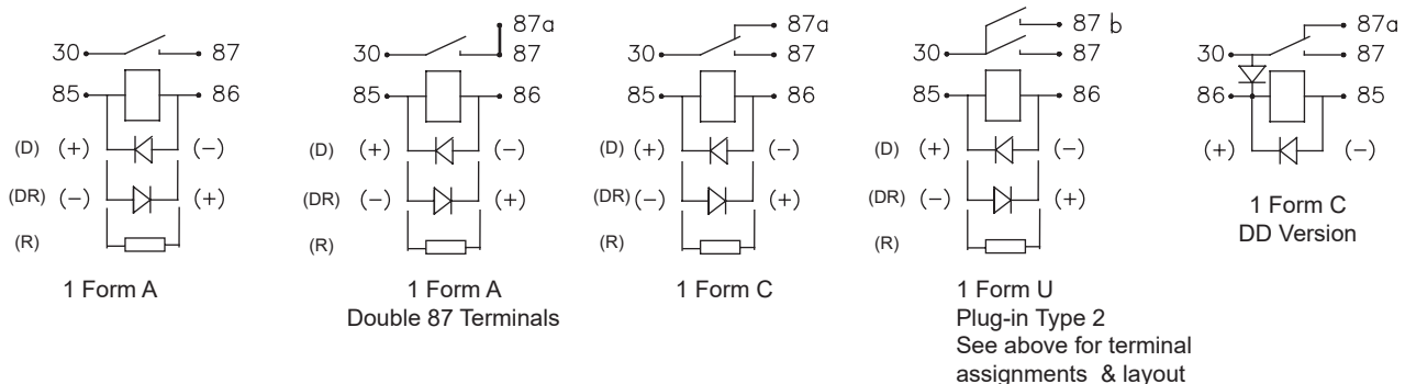
Connection diagrams
