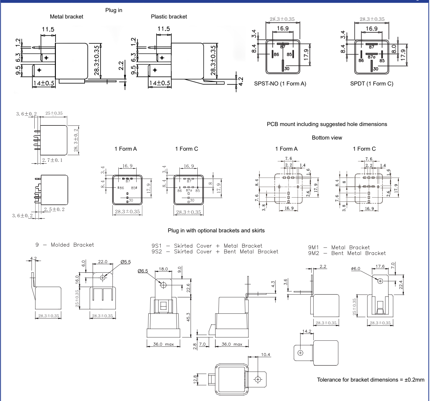
Dimensions mm
