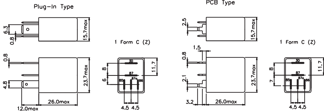
Dimensions mm
