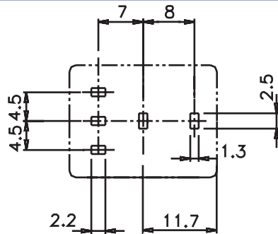
PCB Mounting Dimensions mm
