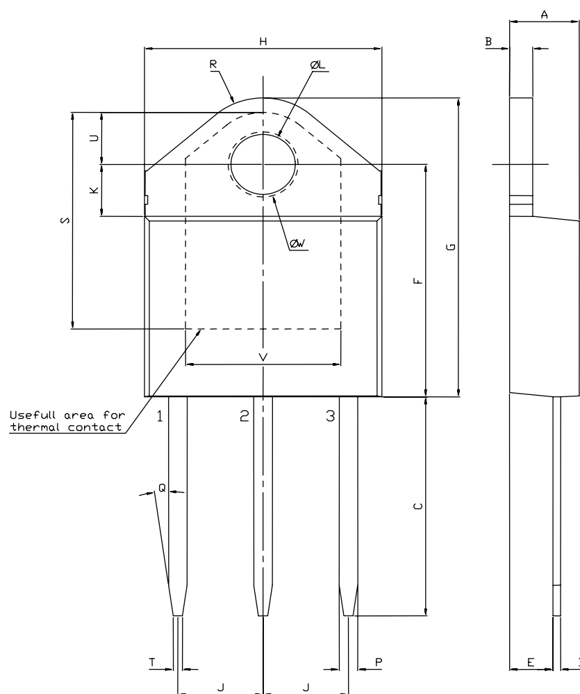
Figure 14. Package outline
