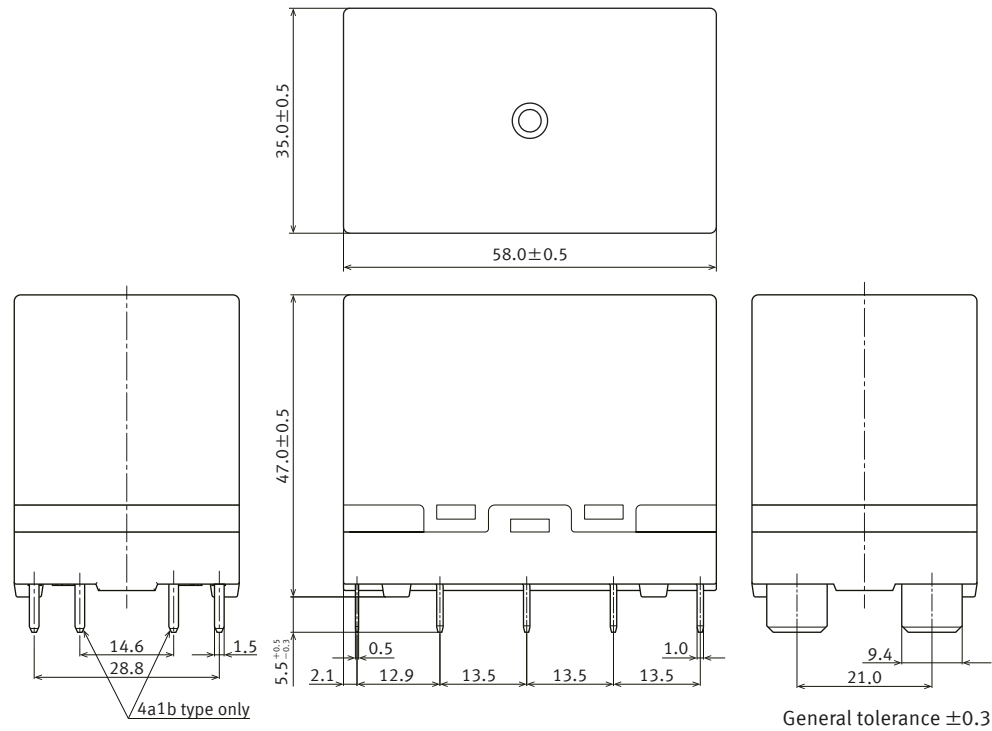
External dimensions
