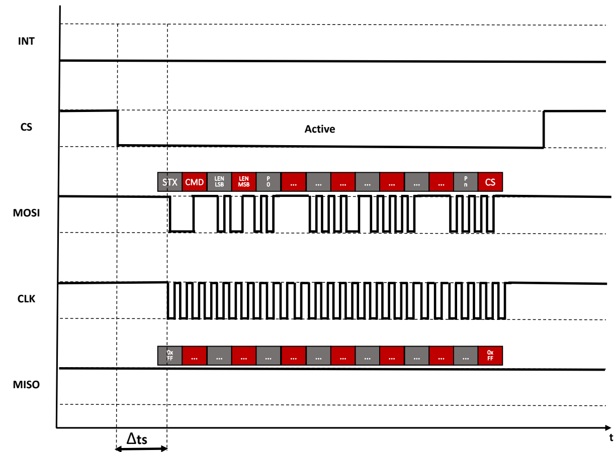
Figure 9: SPI master to slave communication, example SPI_INT "active high"
