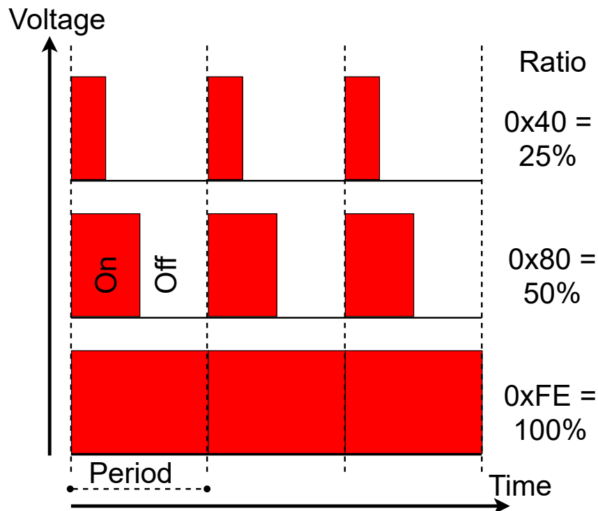
Figure 20: PWM behaviour
