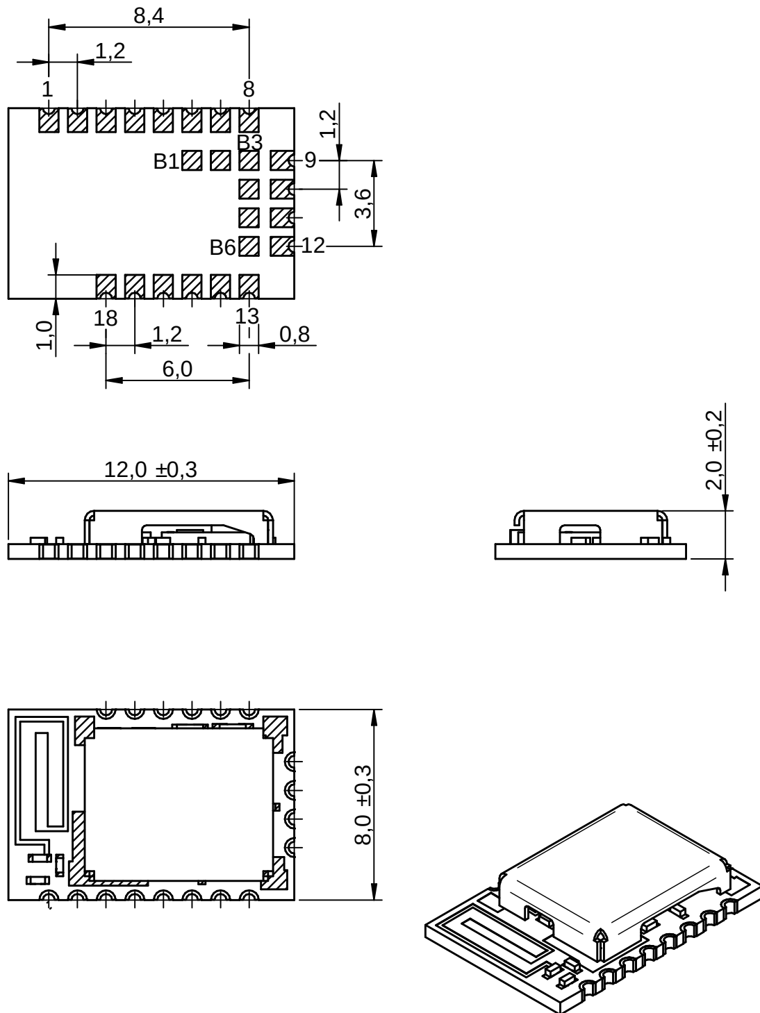
Figure 35: Module dimensions [mm]
