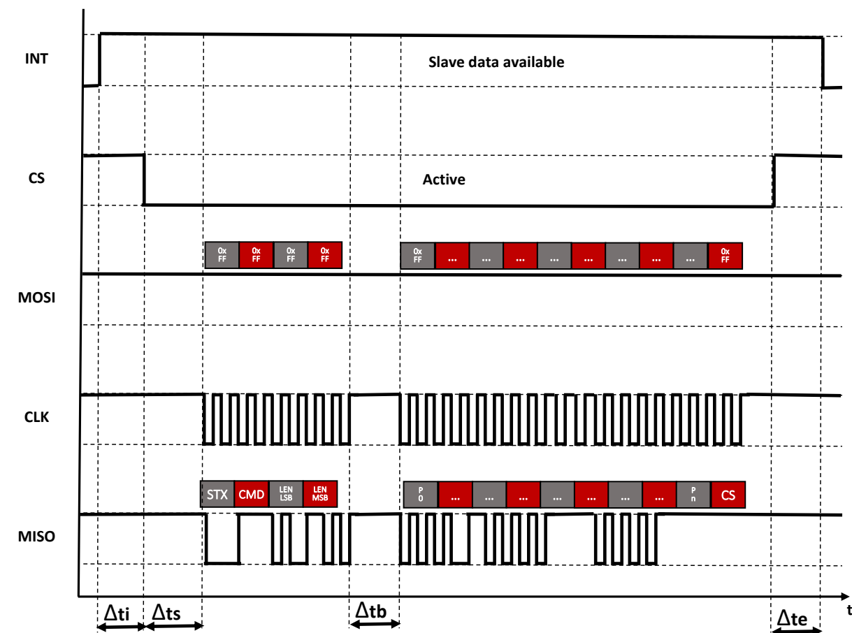
Figure 10: SPI slave to master communication, example SPI_INT "active high"
