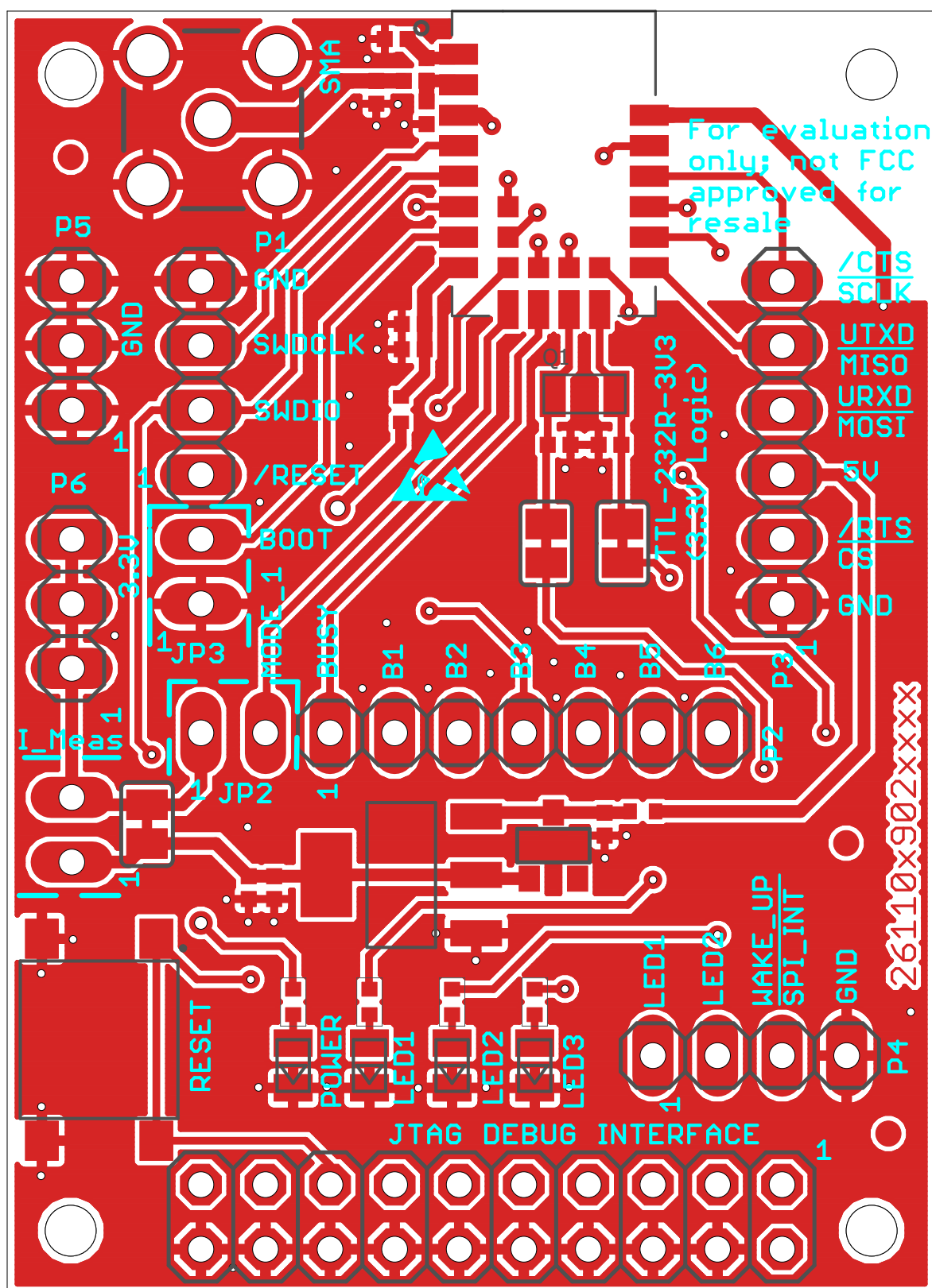
Figure 27: Reference design: Layout
