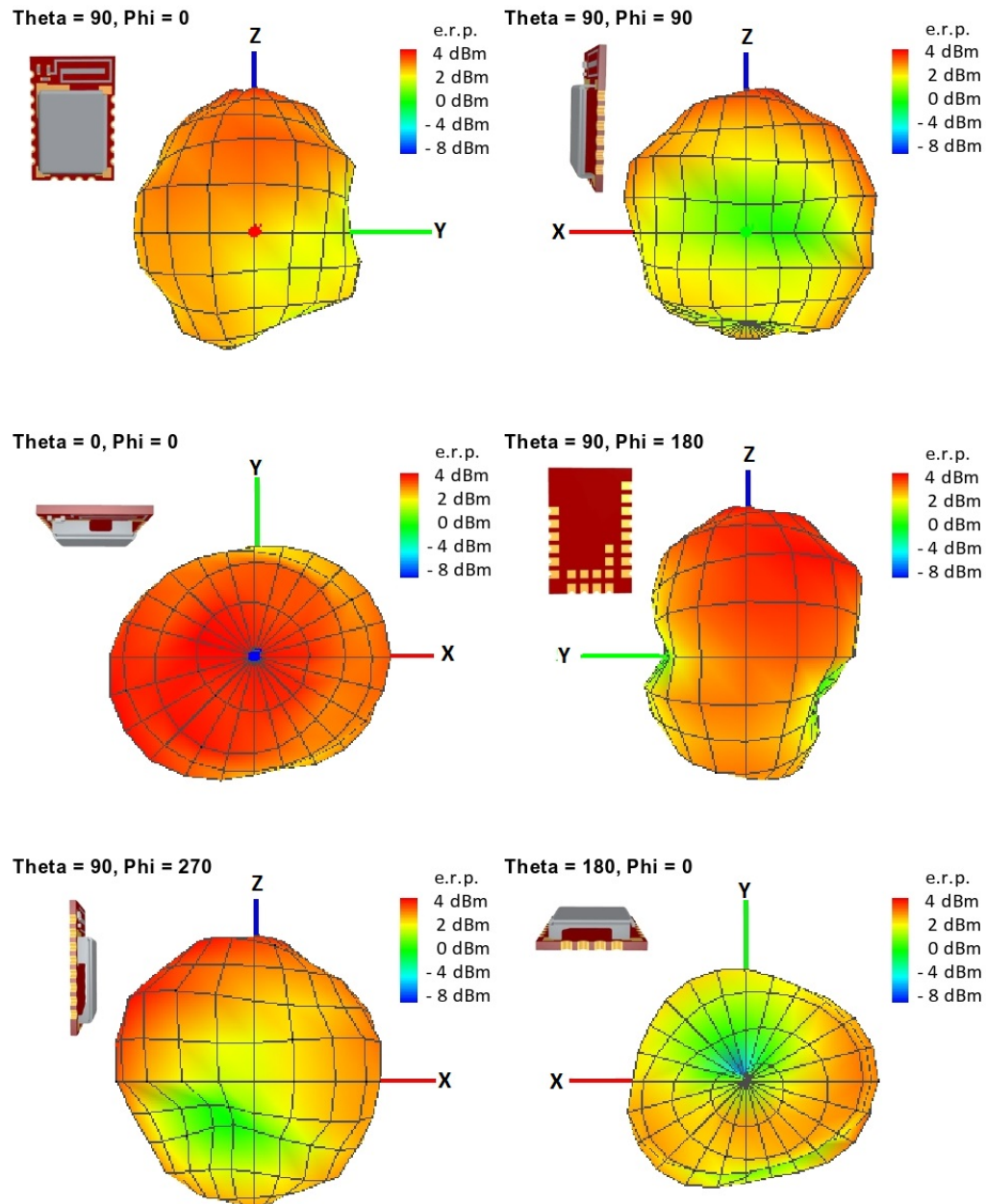
Figure 28: Antenna characteristic of the module with its integrated antenna measured on the official evaluation board (2611149024011)
