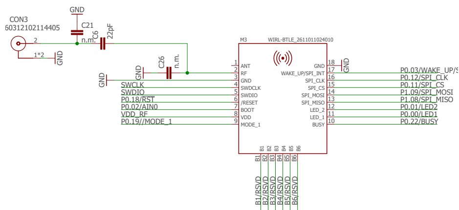
Figure 33: External antenna connection
