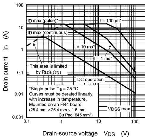
Fig. 8.11 Safe Operating Area
