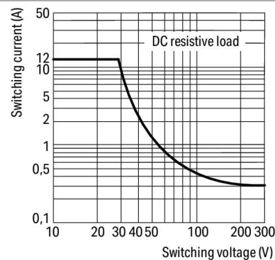
DC load limit curve
