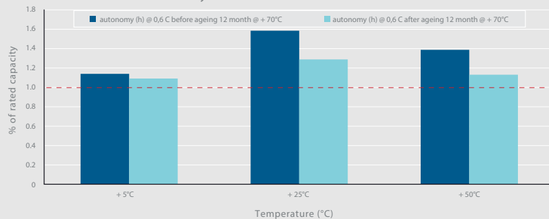
12 months at +70°C simulates 4 years at +50°C
