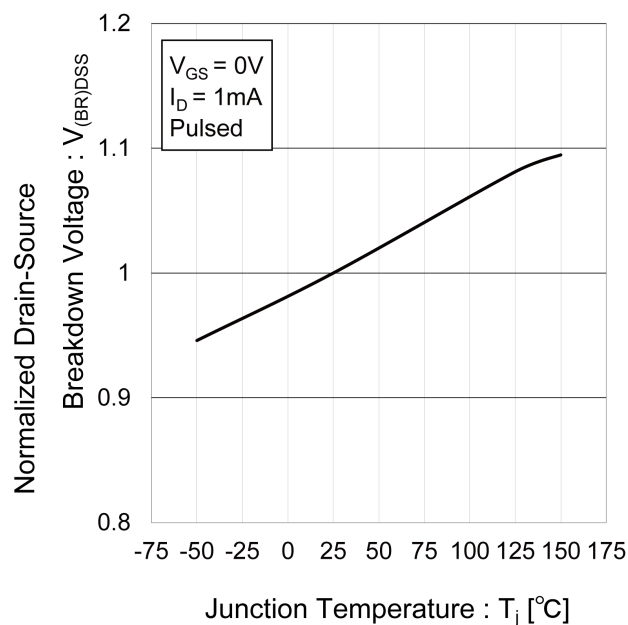
Fig.6 Normalized Breakdown Voltage vs. Junction Temperature
