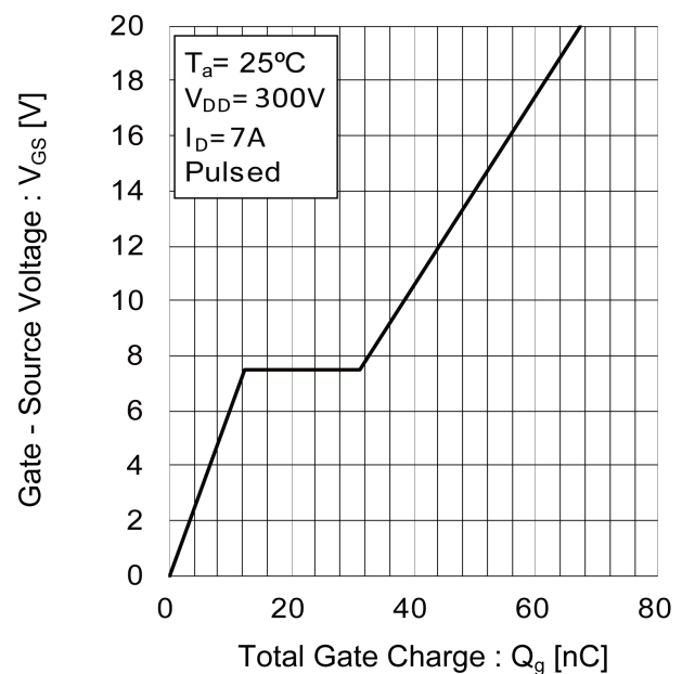
Fig.16 Gate charge
