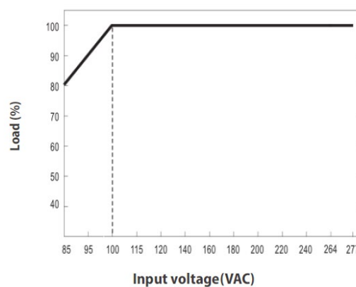
Minus Output and Input Voltage Curves
