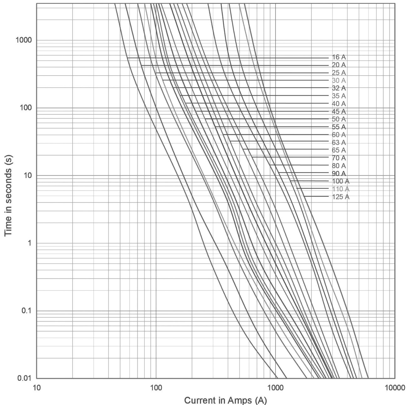
gG Average Current Curve(I-T Curve)
