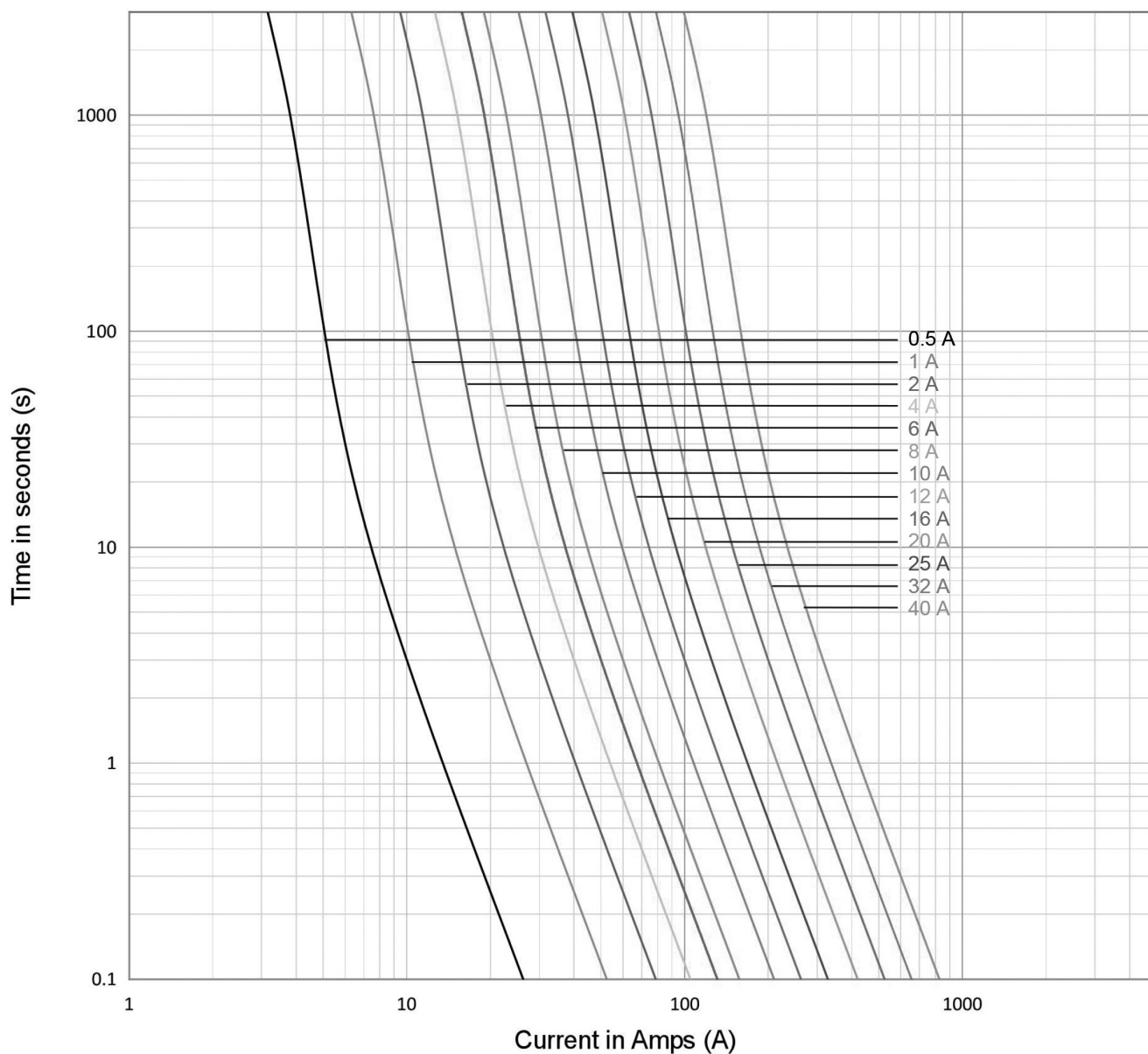
gG Average Current Curve(I-T Curve)
