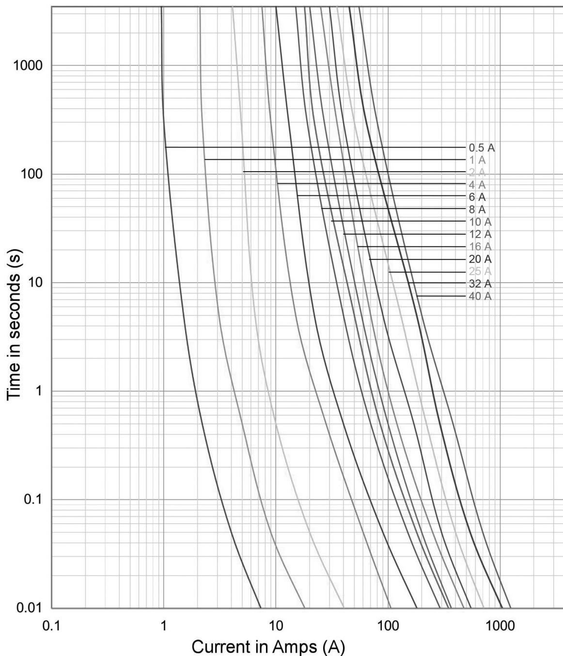
aR Average Current Curve(I-T Curve)
