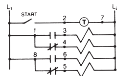
TYPICAL CIRCUIT
