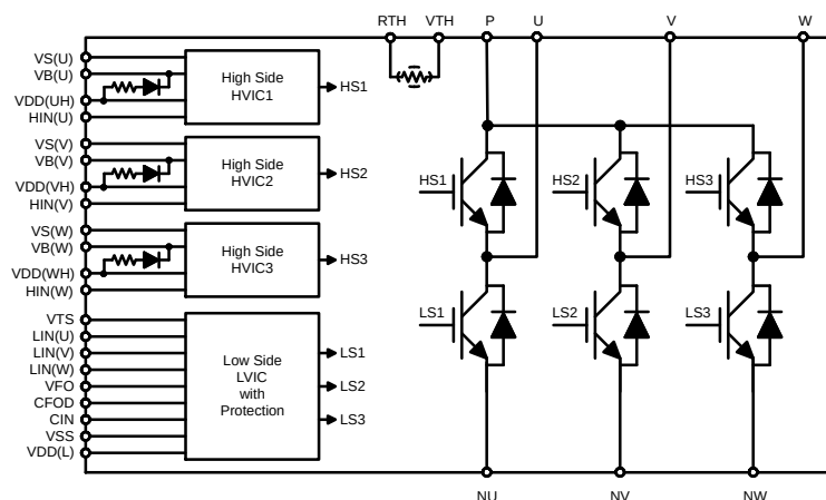
Figure 1. Application Schematic
