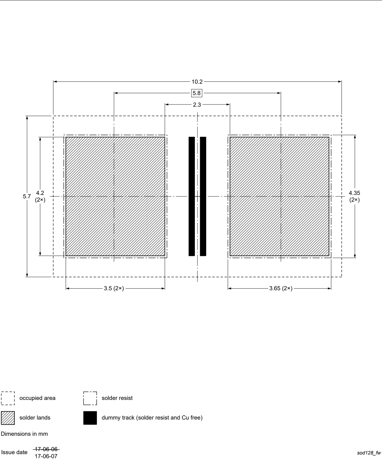
Fig. 17. Wave soldering footprint for CFP5 (SOD128)
