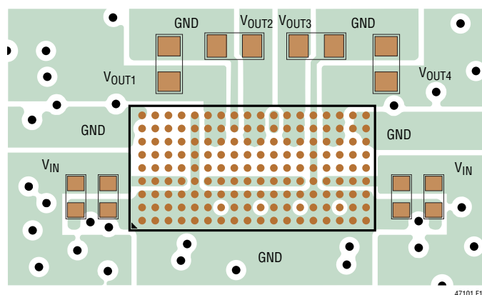
Figure 16. Recommended PCB Layout
