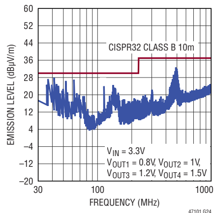
Radiated Emissions 8A Load on Each Channel DC3164A-B, without Ferrite Bead
