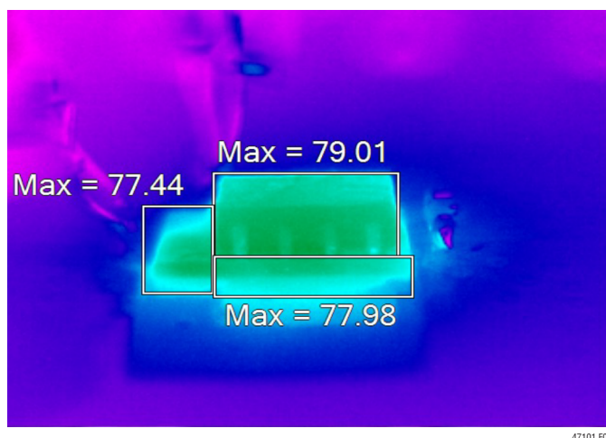
Figure 4. Thermal Image, LTM4710-1 Running from 3.3V Input to 0.5V, Paralleled 32A Output with No Airflow, No Heat Sink
