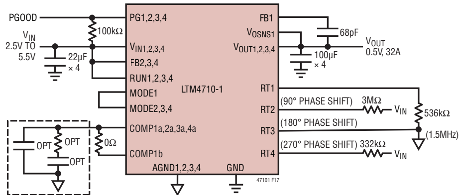
Figure 17. Paralleled Single Output, 32A DC/DC \mu Module Regulator
