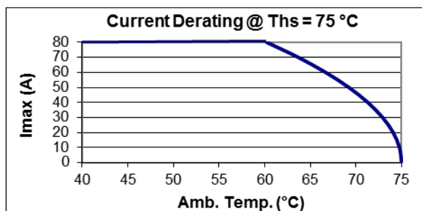
B25620B0268K703
