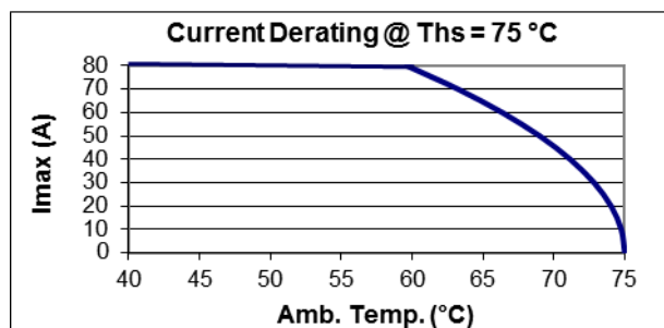
B25620B0198K703
