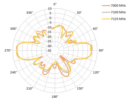
Phi 90° Plane
