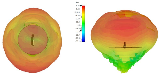
Radiation Patterns at 2700 MHz
